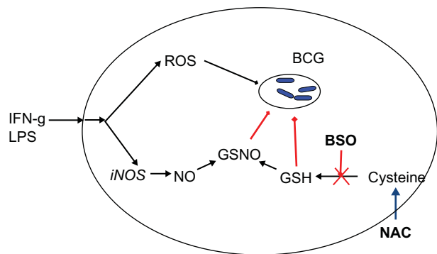
Figure 5 Glutathione in the defense against mycobacterial infections.
