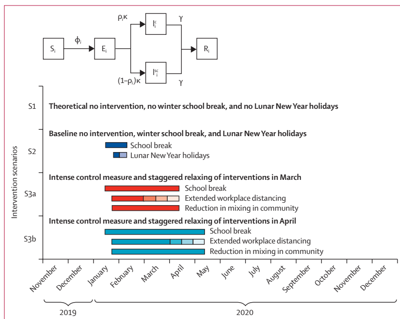
Figure 1: Age-structured SEIR model and details of the modelled physical distancing interventions
